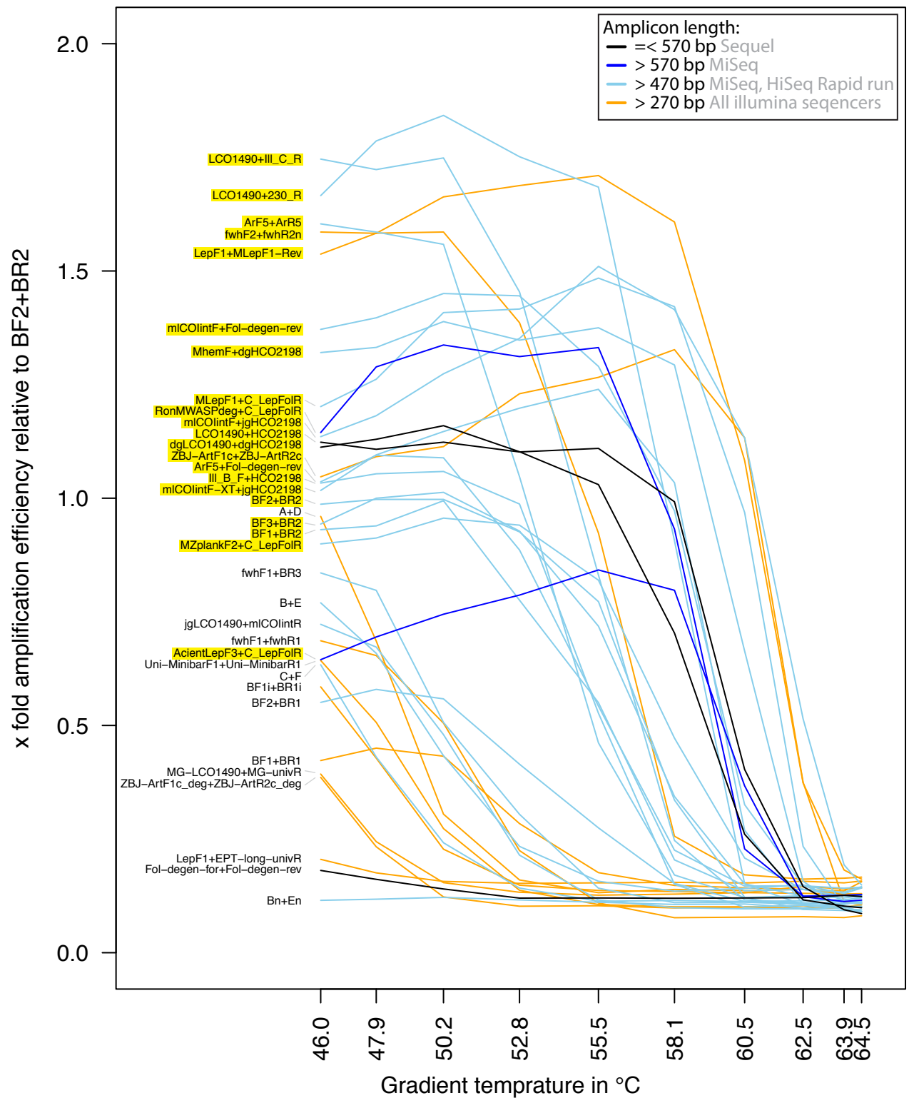
Figure S8: PCR product concentration plotted relative to BF2+BR2 positive control in each sample as different annealing temperatures and 30 PCR cycles. Primer pairs highlighted in Yellow were selected for MiSeq sequencing. Based on the amplicon length the suitability for specific primer combinations for different sequencers is indicated by the line color.
