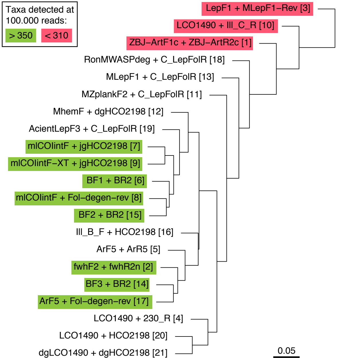
Figure S14: Cluster Dendrogram (UPGMA) for Jaccard similarity (A) and Bray-Curtis dissimilarity (B) for the mock sample metabarcoding data using 21 primer sets, generated with the R package veagan v2.5-2. If the number of taxa detected is above 350 or below 310 taxa, the primer set is highlighted in Green or Red respectively. Sequencing depth was normalised to 100.000 reads for each primer sets (reads below 0.001% abundance discarded).
