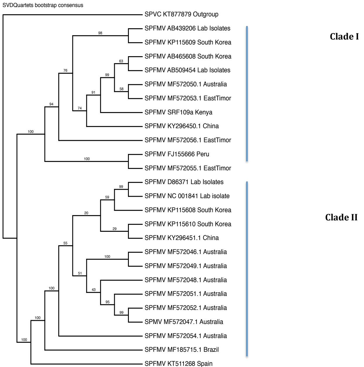
Fig. S5. Species tree generated from SVD Quartets using the complete genome of Sweet potato feathery mottle virus (SPFMV) sequences with bootstrap support of branches.
