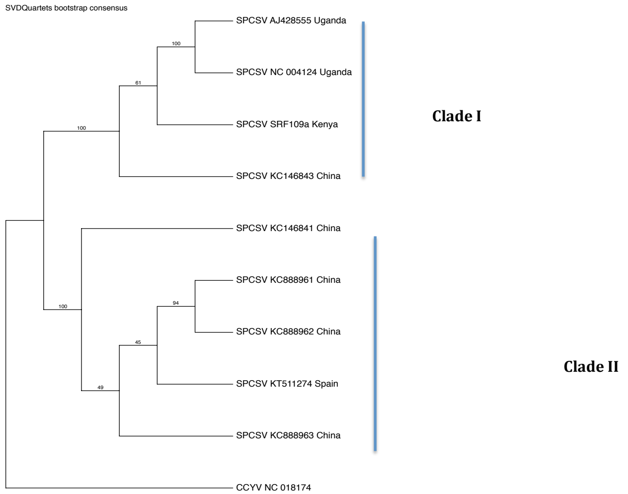
Fig. S1 Species tree generated from SVD Quartets using the complete genome RNA1 of sweet potato chlorotic stunt virus (SPCSV VIRUS) sequences with bootstrap support of branches.
