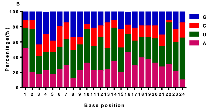
A: miRNA nucleotide bias of the first base B: miRNA nucleotide bias at each position Supplementary Fig3. miRNA nucleotide bias in amaranthus
