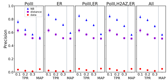
(b) test data performance
