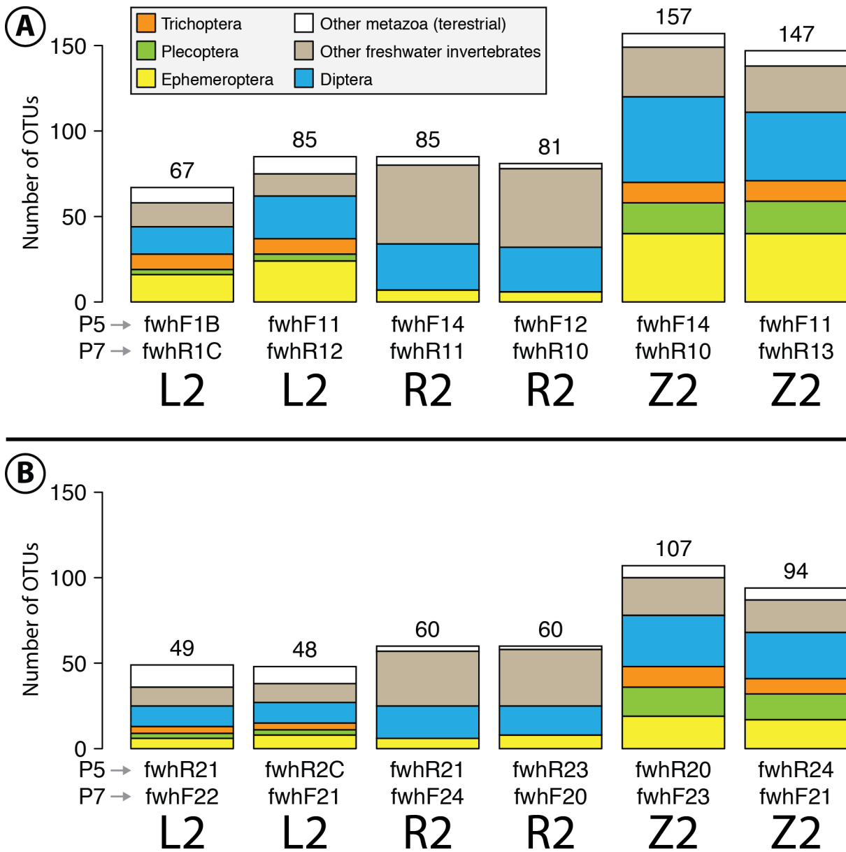
Figure S7: Bar plot showing the OTU composition of samples and replicates for key macroinvertebrate orders.
