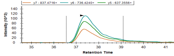
Spectral library
