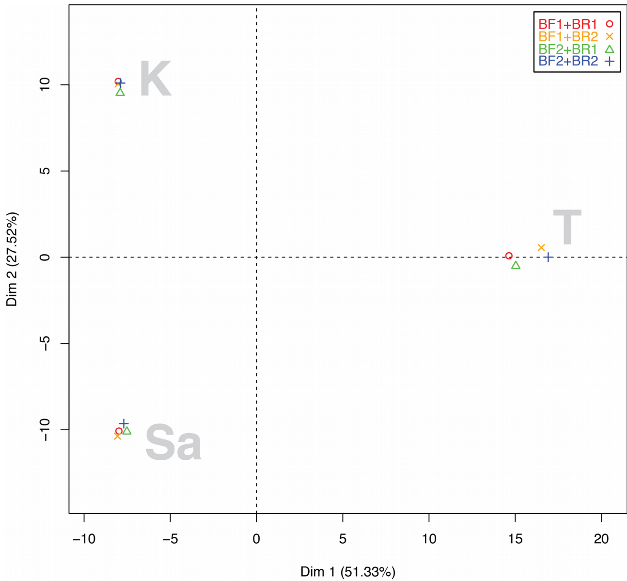
Figure S9: Principal component analysis (PCA) on macroinvertebrates detected with DNA metabarcoding (presence / absence) across the 3 stream types detected with all different 4 primer combinations. Sa = clayish catchments, K = mineral land catchments, T = peatland catchments.
