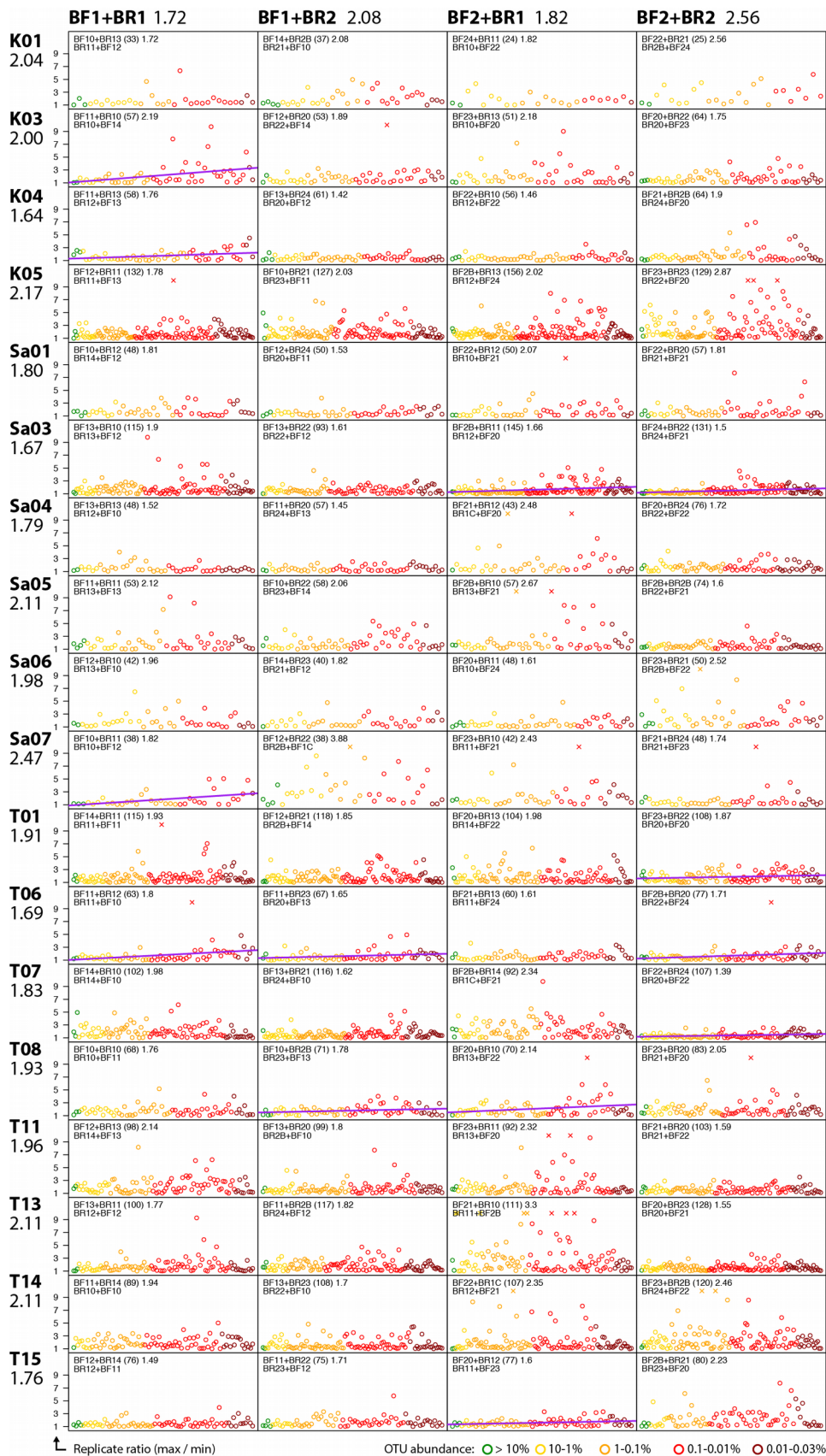
Figure S6: Difference between OTU abundance between replicates sorted by read abundance indicated by color. If the ratio of maximum divided by minimum read abundance exceeds 10 the data point is plotted as an “x”. The total number of OTUs per sample is given in brackets, followed by the mean ratio. The mean ratio for rows and columns is given below the sample ID or right of the primer combinations.
