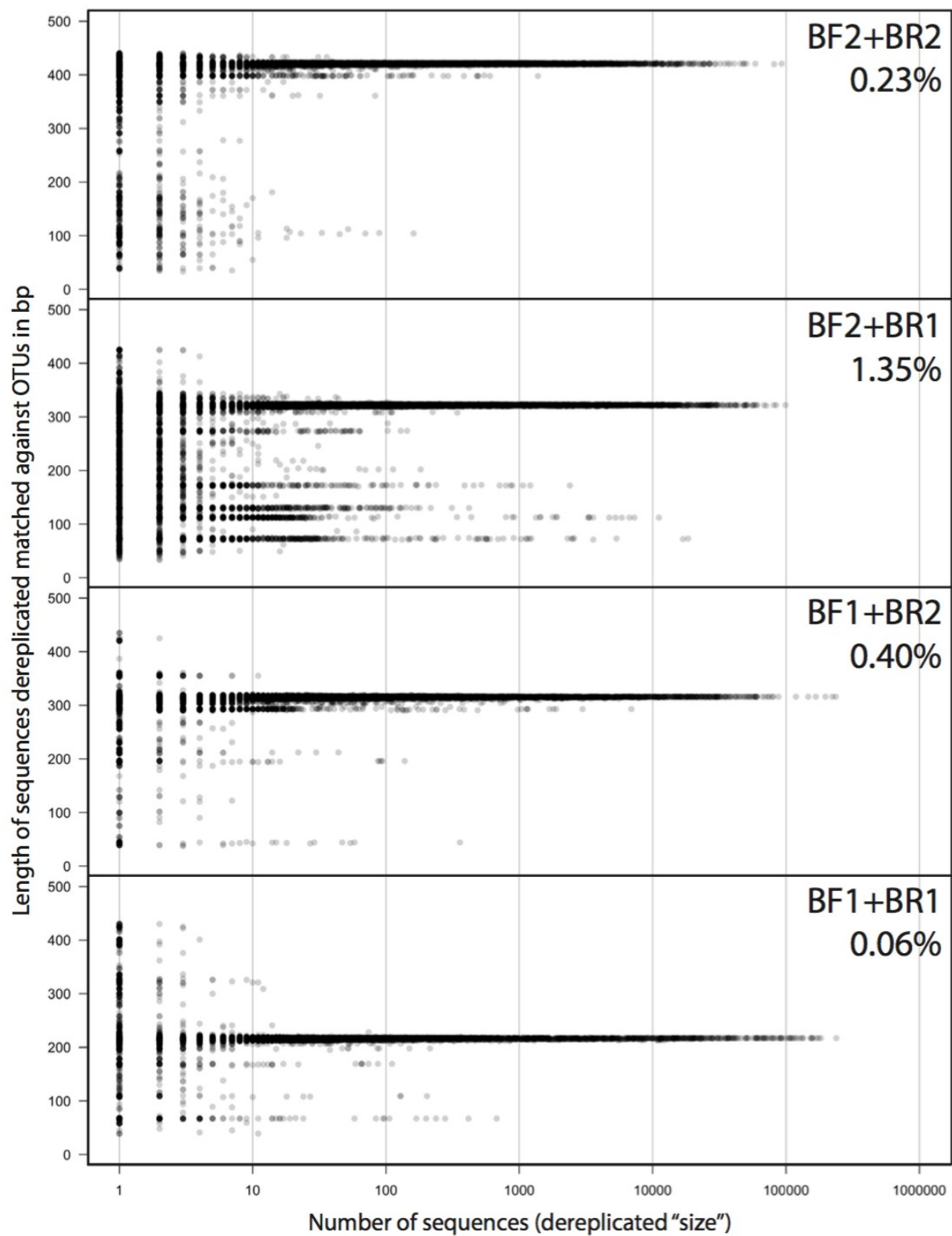
Figure S7: Length distribution and abundance of individual sequences assigned to each OTU for all primer combinations. The percentage value indicates the proportion of sequences which are at least 10 bp longer or shorter than the expected amplicon length.
