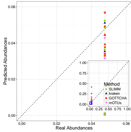
(b) HMP-mock-ill-even
