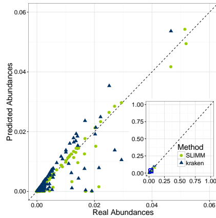
(h) CAML_M2-S002
