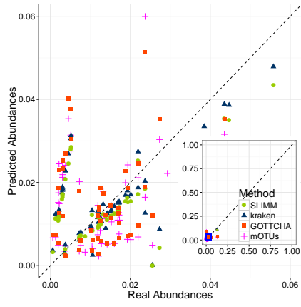
(a) AB-64
