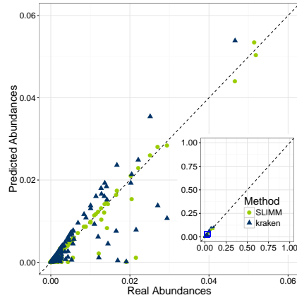
(f) CAML_M1-S002
