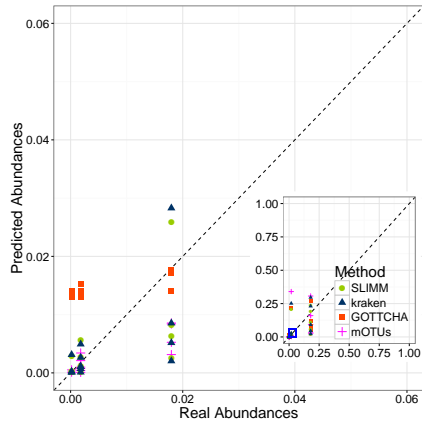
(c) HMP-mock-ill-stag
