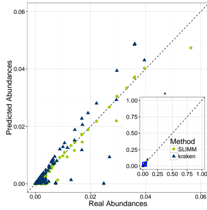
(g) CAML_M2-S001
