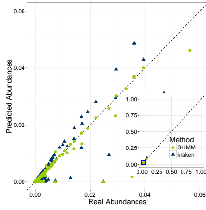
(e) CAML_M1-S001
