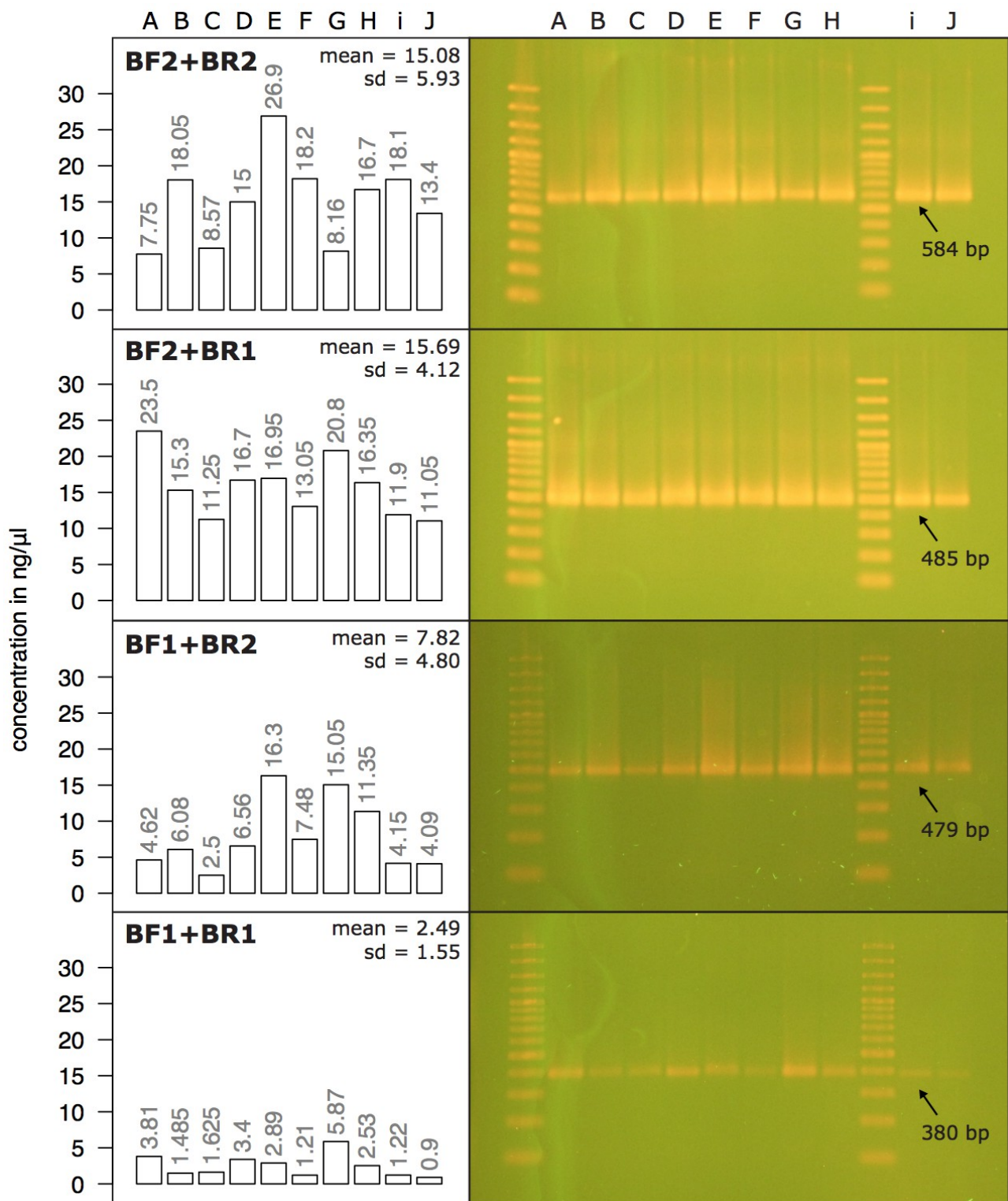
Figure S5: Overview of obtained products after one-step PCR and magnet bead clean up. Fragment concentrations were measured using the Qbit HS kit.
