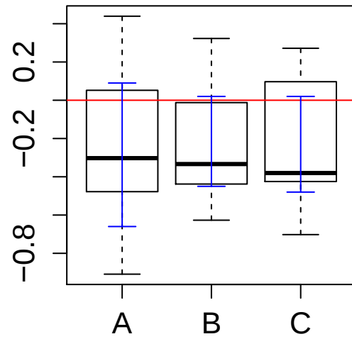
Elevation total effect
