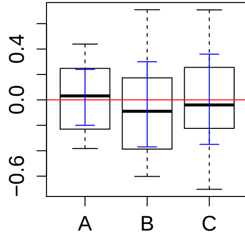
Flower diversity total effe
