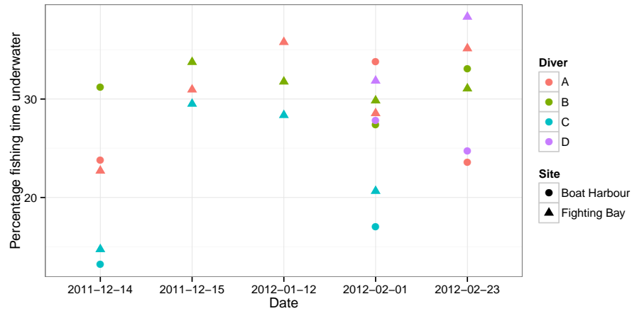
Figure C-2. Ratio of time spent underwater to time spent fishing, for each diver (A–D) at the unfished site at Fighting Bay (closed to fishing in 1996) and the fished site at Boat Harbour, New Zealand, over the course of the fish-down experiment.
