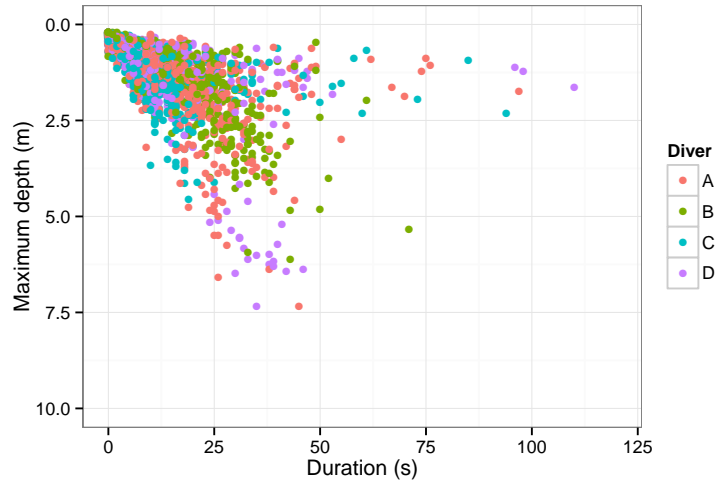
Figure C-1. Relationship between maximum dive depth and dive duration, for each of the four divers (A–D) diving for abalone (pāua, Haliotis iris ) during the fish-down experiment at Fighting Bay, New Zealand in 2011–12.
