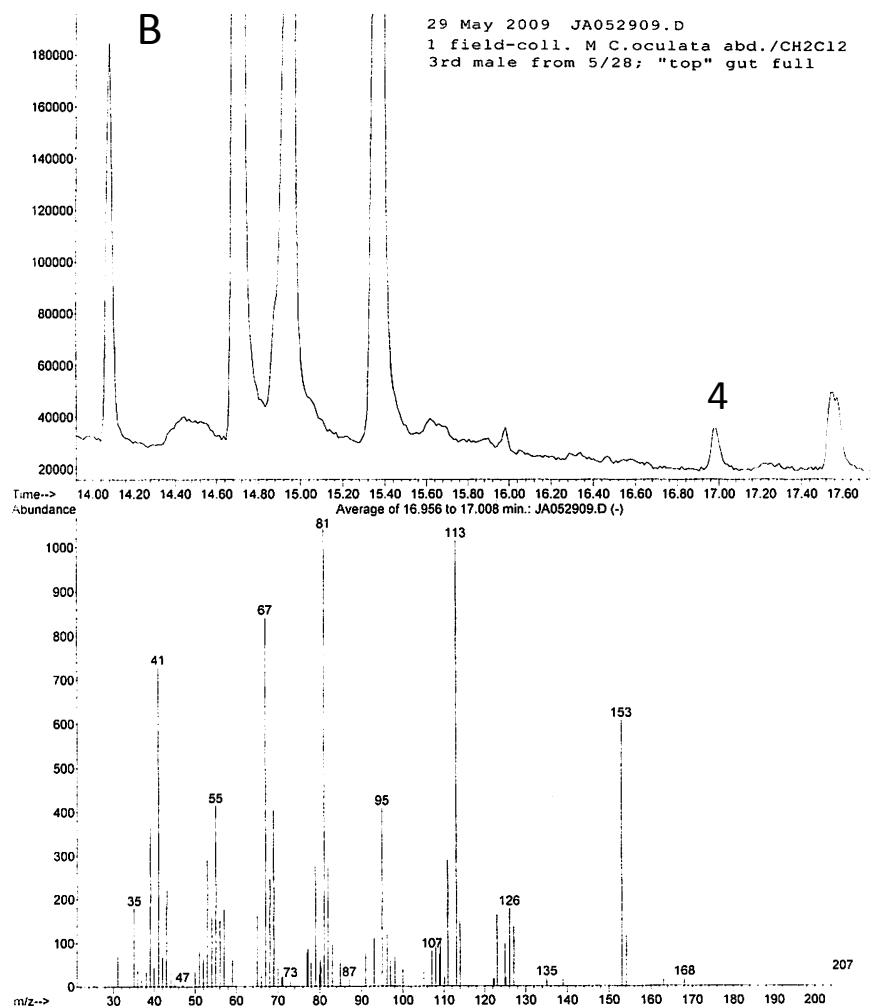
Suppl. Figure 2 GC and MS data of abdominal cuticular extracts from Chrysopa Oculata males a) & b) collected 28 May, 2009, sweeping vetch, Beltsville, MD. (4 = dihydronepetalactone (column = 30m HP-5; conditions described in text))
