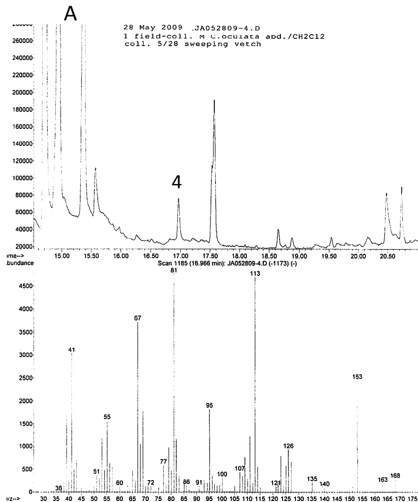
Suppl. Figure 2 GC and MS data of abdominal cuticular extracts from Chrysopa Oculata males a) & b) collected 28 May, 2009, sweeping vetch, Beltsville, MD. (4 = dihydronepetalactone (column = 30m HP-5; conditions described in text))
