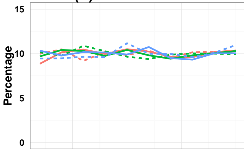
(A) 3 variables
