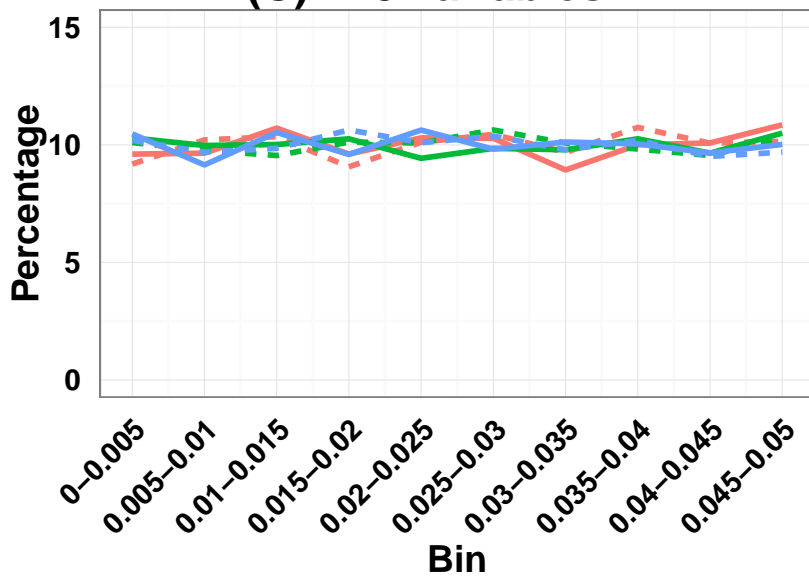
(C) 8 variables
