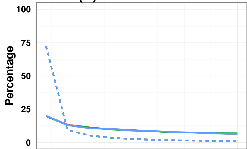
(B) 3 variables
