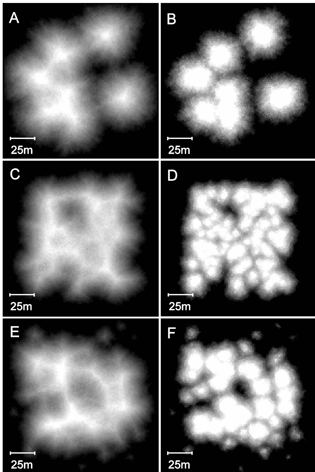
Plan views of model branching and massive coral reefs, showing the effects of decreasing the recruitment rate from 0.25% to 0.125% ( A – branching reef, 100 iterations, and B – massive reef, 80 iterations), increasing the recruitment rate to 1% ( C – branching reef, 90 iterations and D – massive reef, 60 iterations), and periodically adding new recruits during reef growth ( E – branching reef, 100 iterations, and F – massive reef, 70 iterations).
