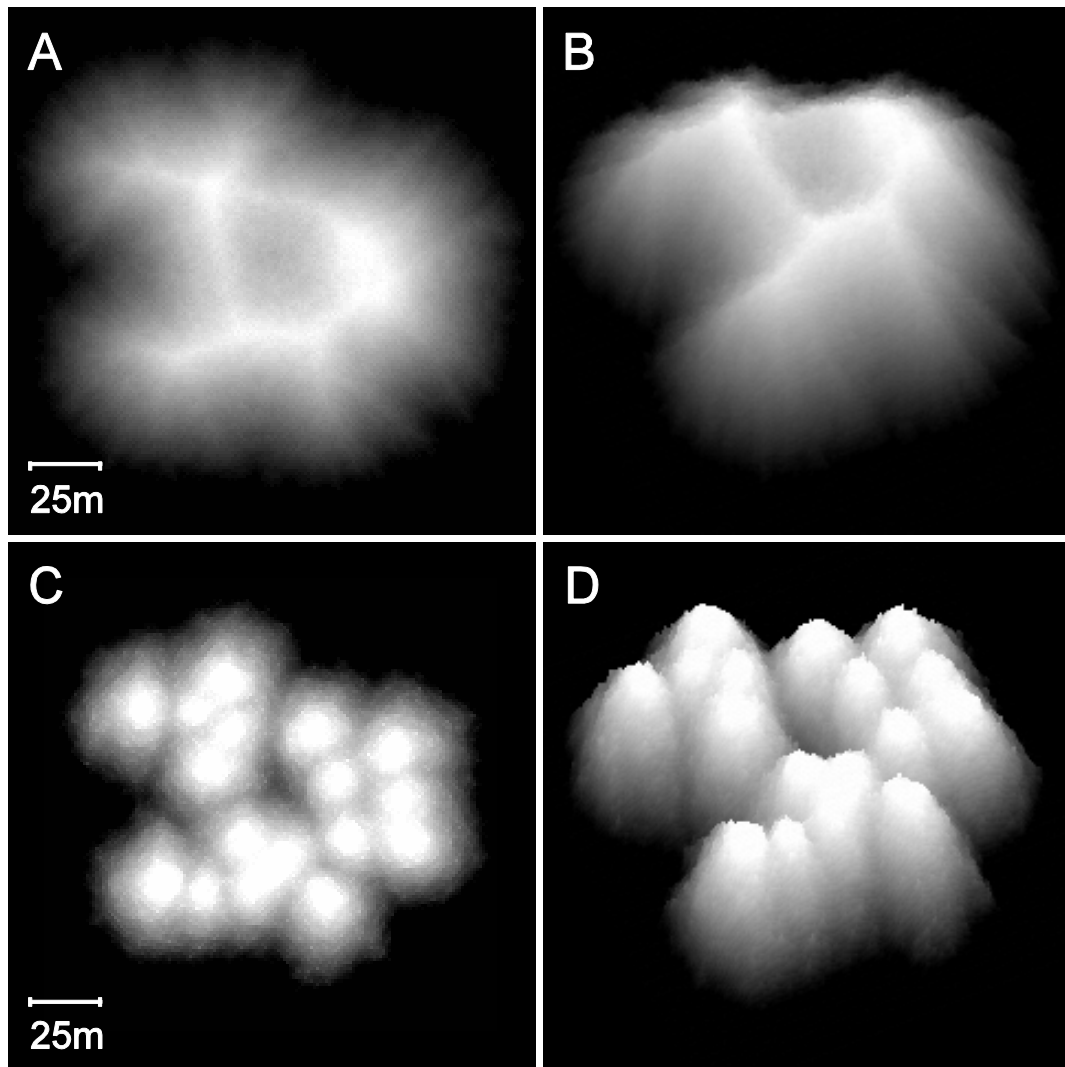
Effect on model reef morphology of increasing water depth to 50m. A) Plan view of branching reef after 150 iterations. B) Oblique view. C) Plan view of massive reef after 100 iterations. D) Oblique view.
